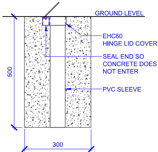
GROUND SLEEVE DETAIL SCALE 1:10
