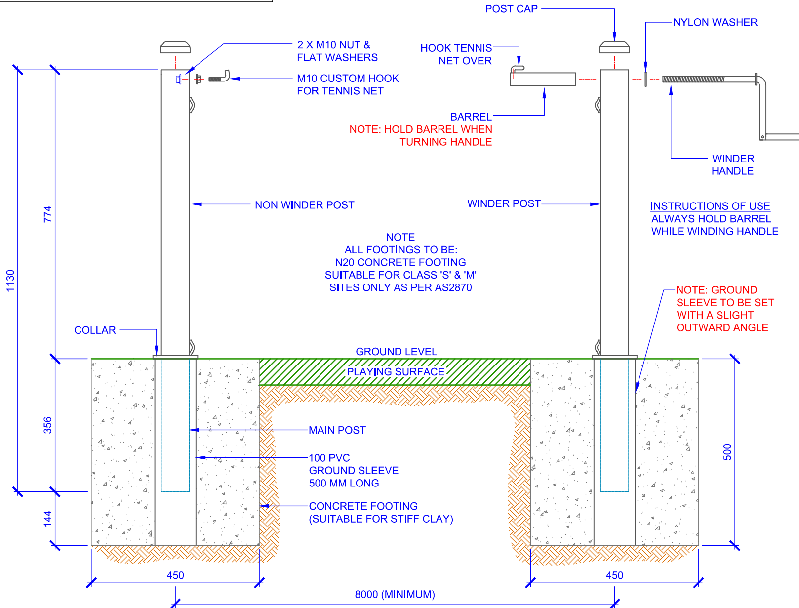
TBW75/2 BARREL WINDER TENNIS POSTS SCALE 1:10
