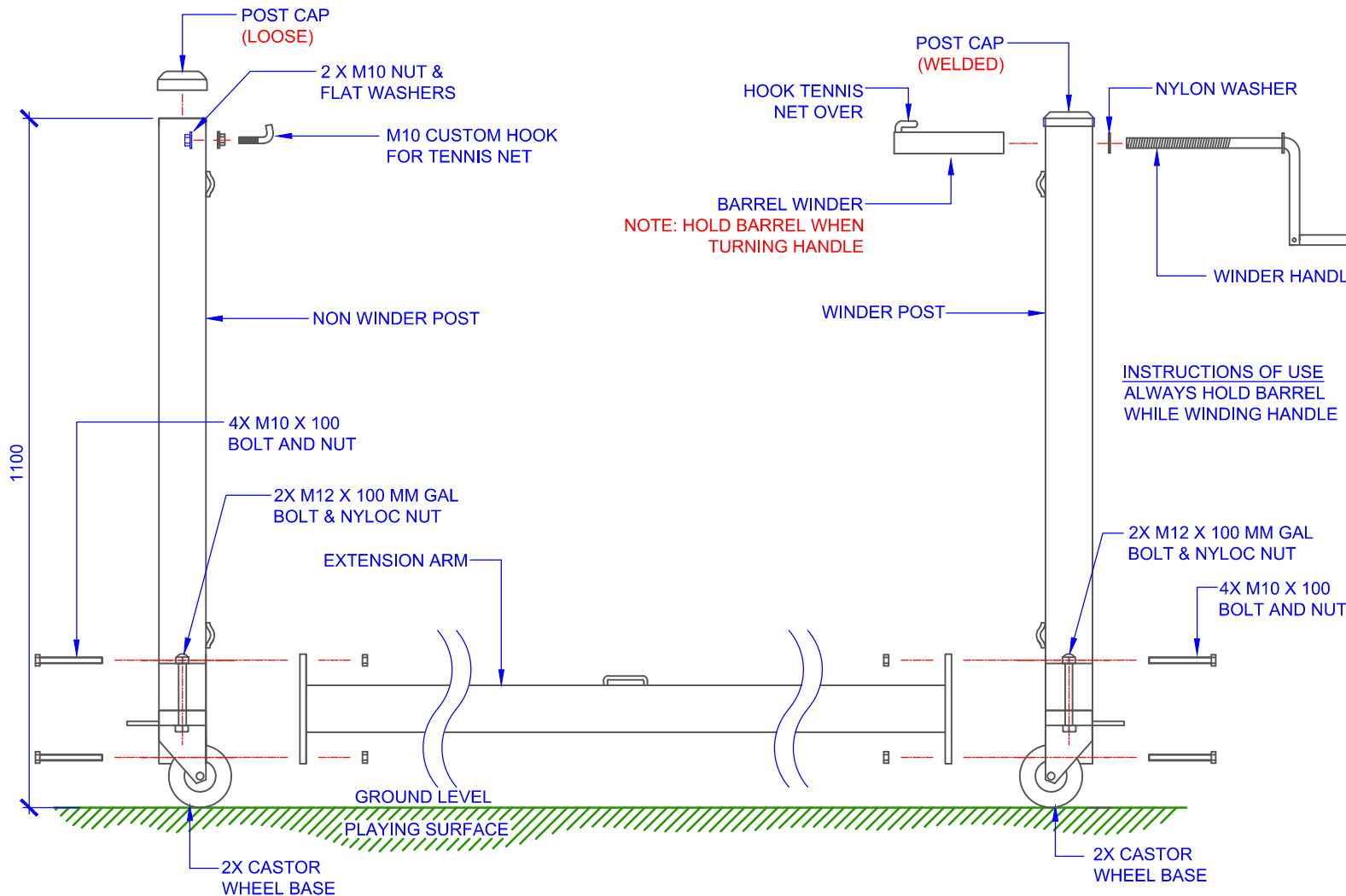
TPF75-BW-2 FREESTANDING NET POSTS SCALE 1:10
