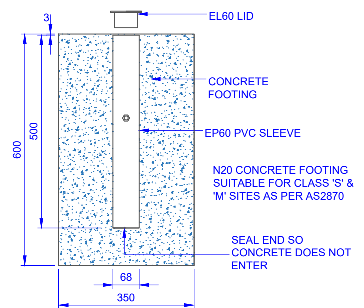
SLEEVE OPTION: EP60 PVC SLEEVE WITH EL60 LOOSE CAP
