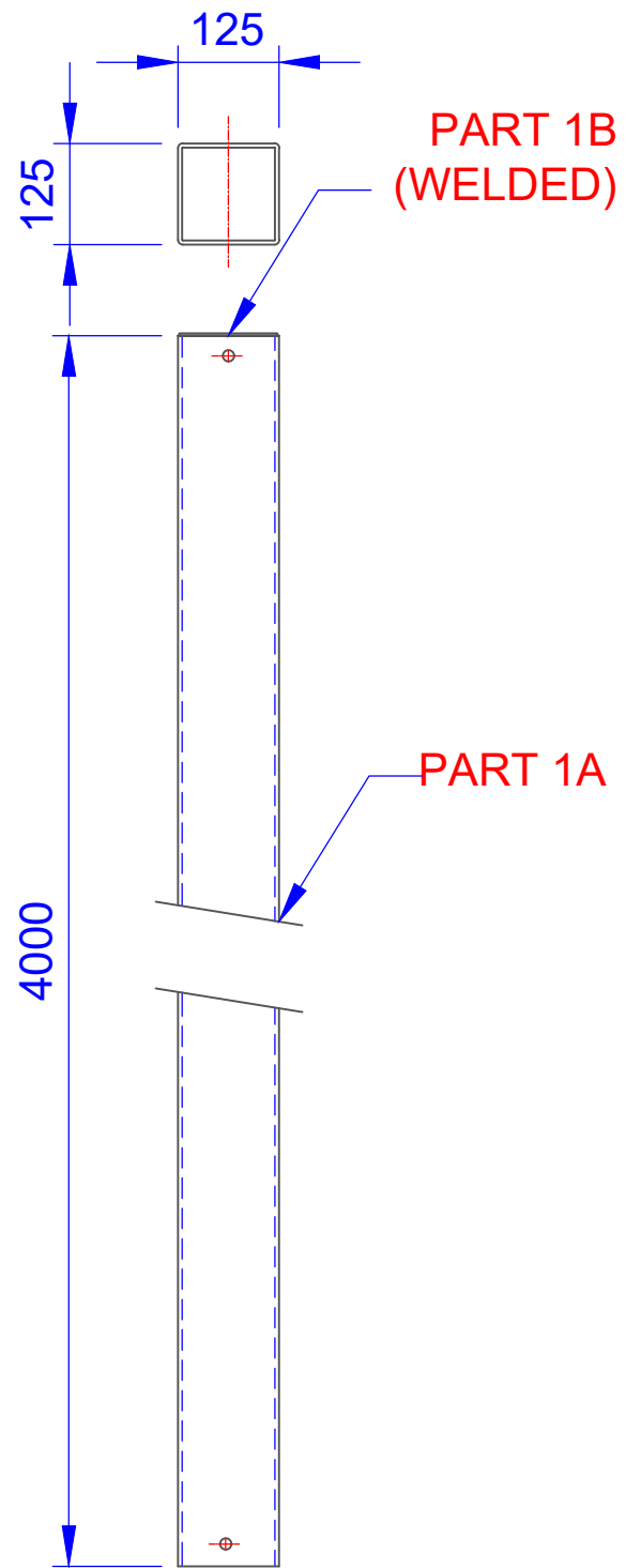
SUB ASSY 01 MAIN POST
