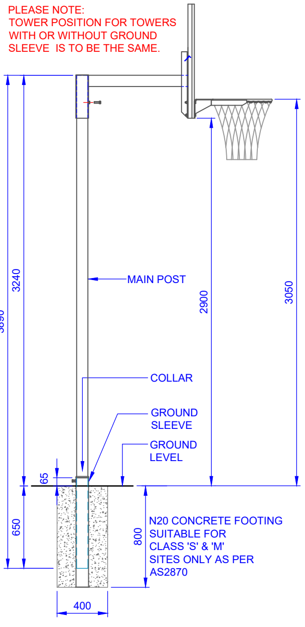
LEGEND BASKETBALL TOWER WITH GROUND SLEEVE SCALE 1:30
