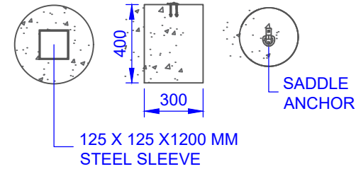
ANCHOR FOOTING B (X10) (F2)
