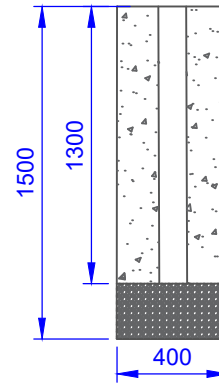
POLE FOOTING A (X3) (F1) FOR SOIL TYPES A, S, M
