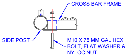
CROSS BAR CONNECTION DETAIL
