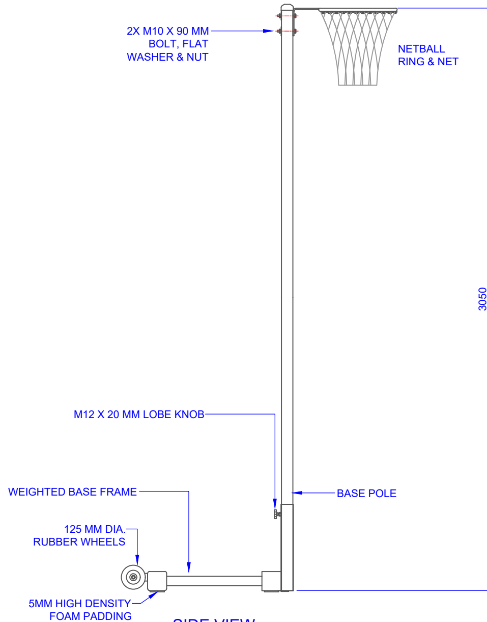
NSP60 PORTABLE NETBALL POST SCALE 1:20
