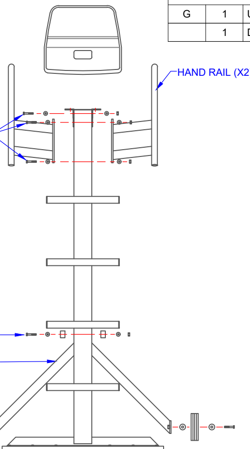
TC25 FRONT VIEW
