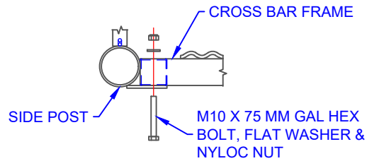
CROSS BAR CONNECTION DETAIL
