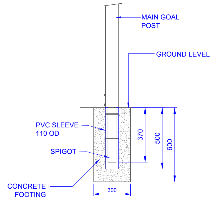
FOOTING DETAIL
