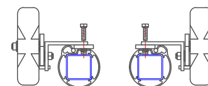
ATTACHING THE WHEELS INTO THE SIDE GROUND BARS
