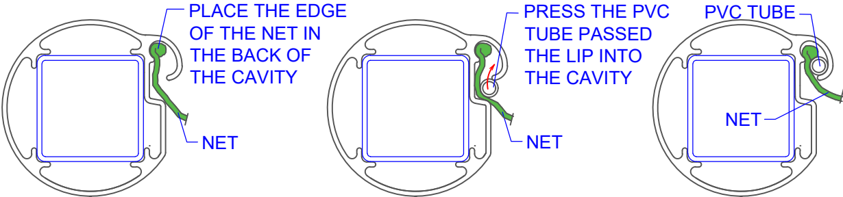
PROCESS TO INSERT THE NET IN THE PROFILE
