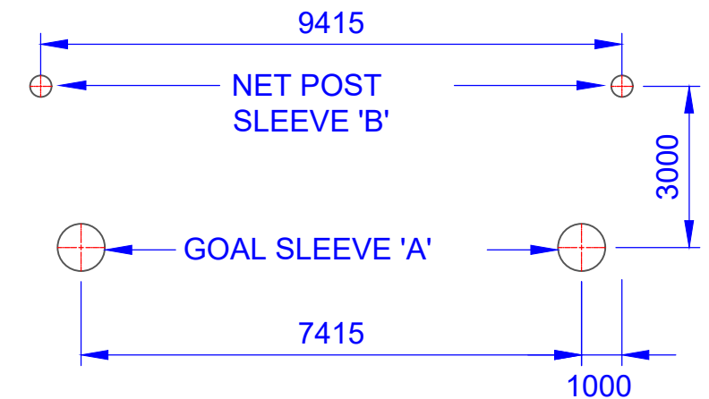
TOP VIEW POST LOCATION SCALE 1:10
