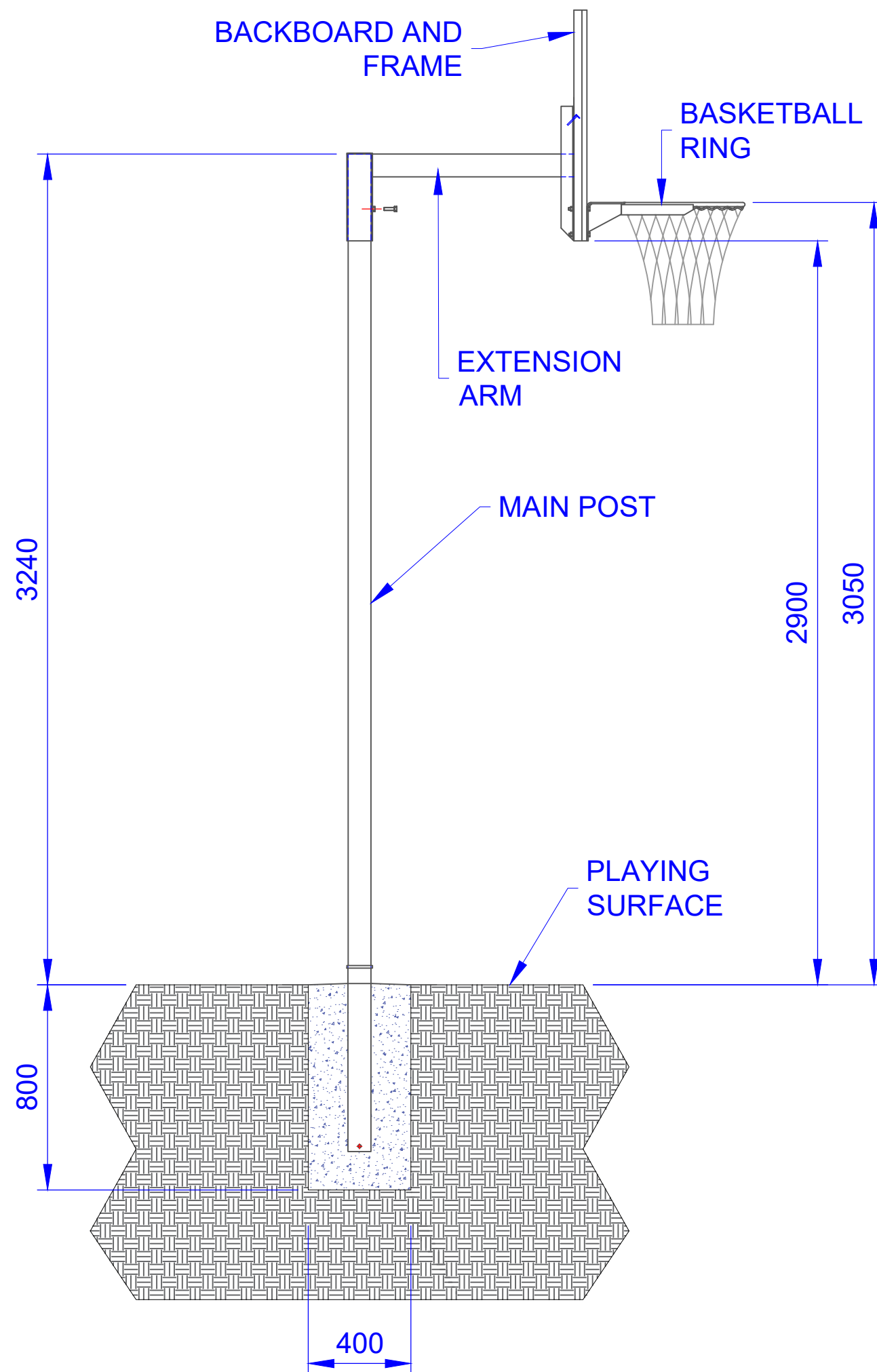
LEGEND BASKETBALL TOWER SCALE 1:20
