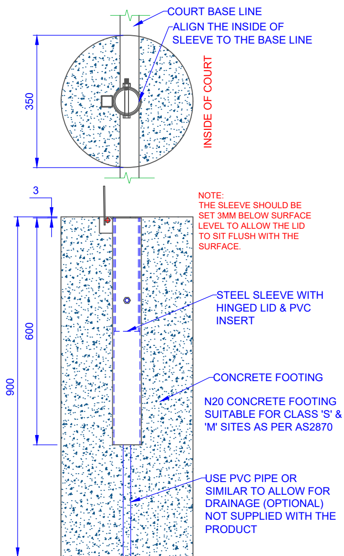
SLEEVE OPTION: EHC60s STEEL SLEEVE WITH HINGED CAP
