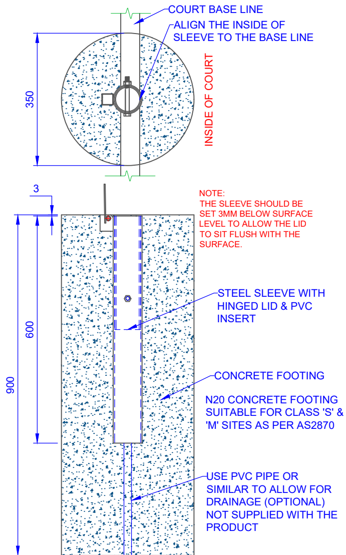
SLEEVE OPTION: EHC60s STEEL SLEEVE WITH HINGED CAP
