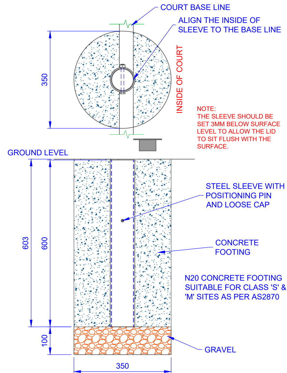
SLEEVE OPTION: ES76 PVC SLEEVE WITH EL76 LOOSE CAP
