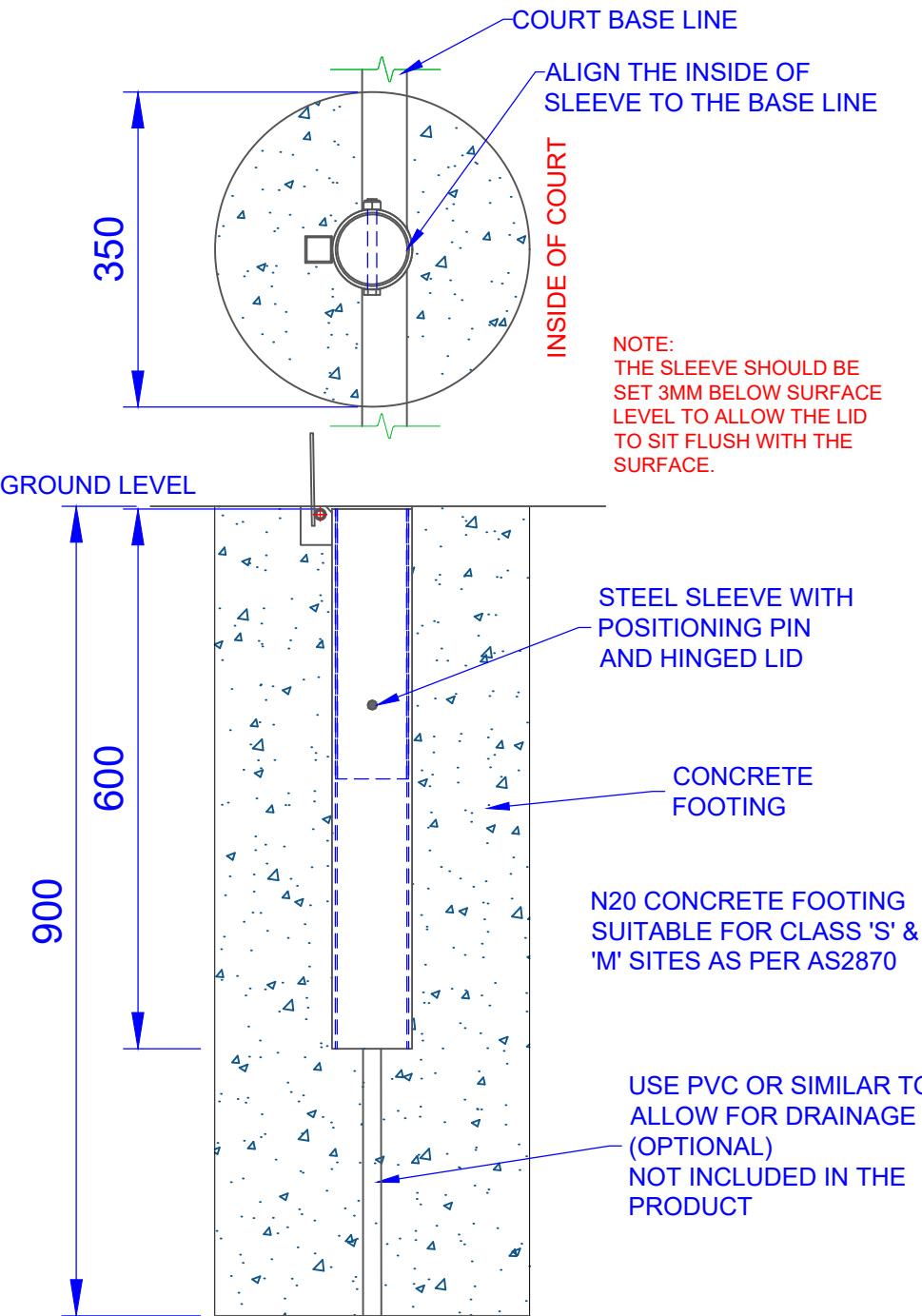
SLEEVE OPTION EHC76 STEEL SLEEVE WITH HINGED LID
