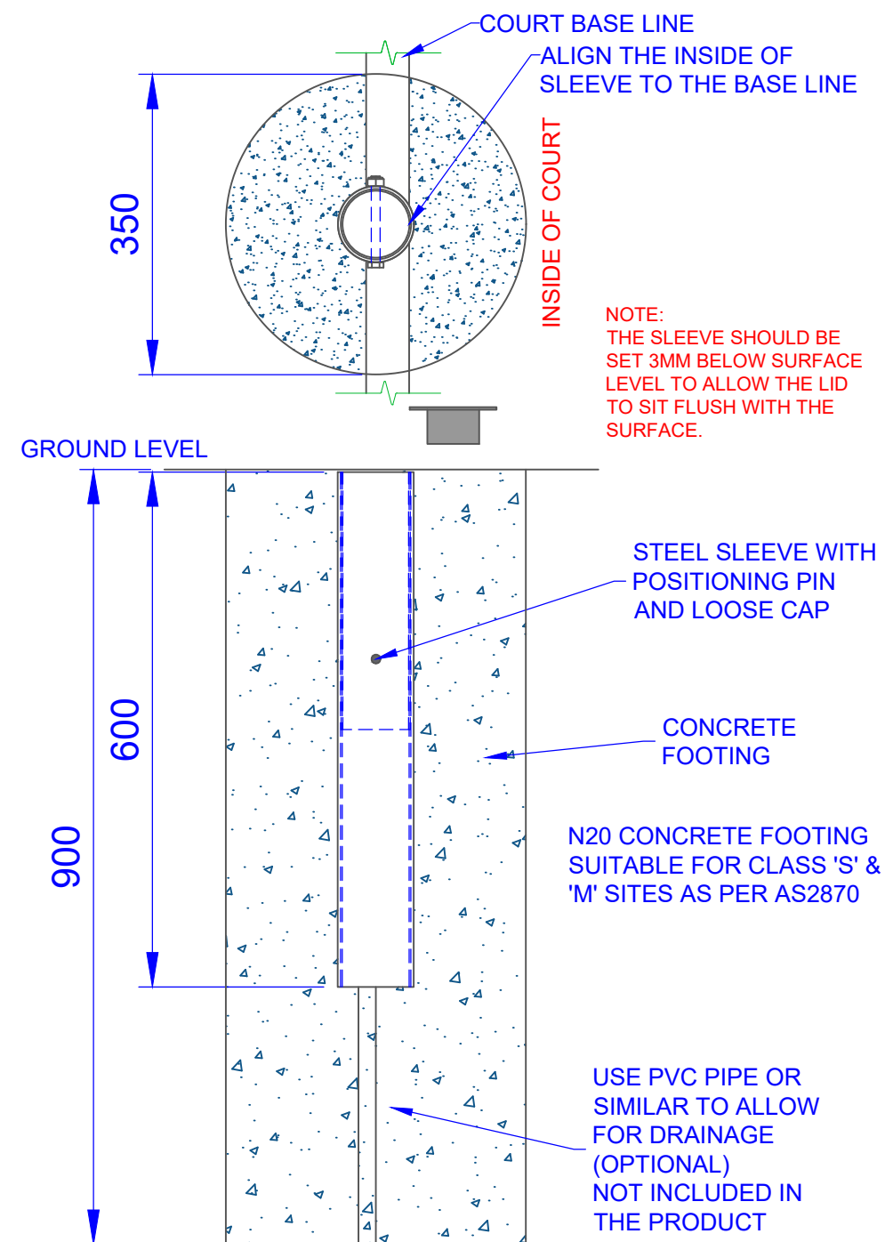
SLEEVE OPTION: ES76 STEEL SLEEVE WITH EL76 LOOSE CAP
