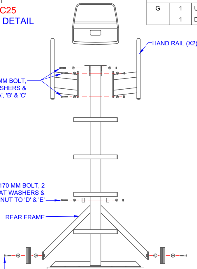
TC25 FRONT VIEW
