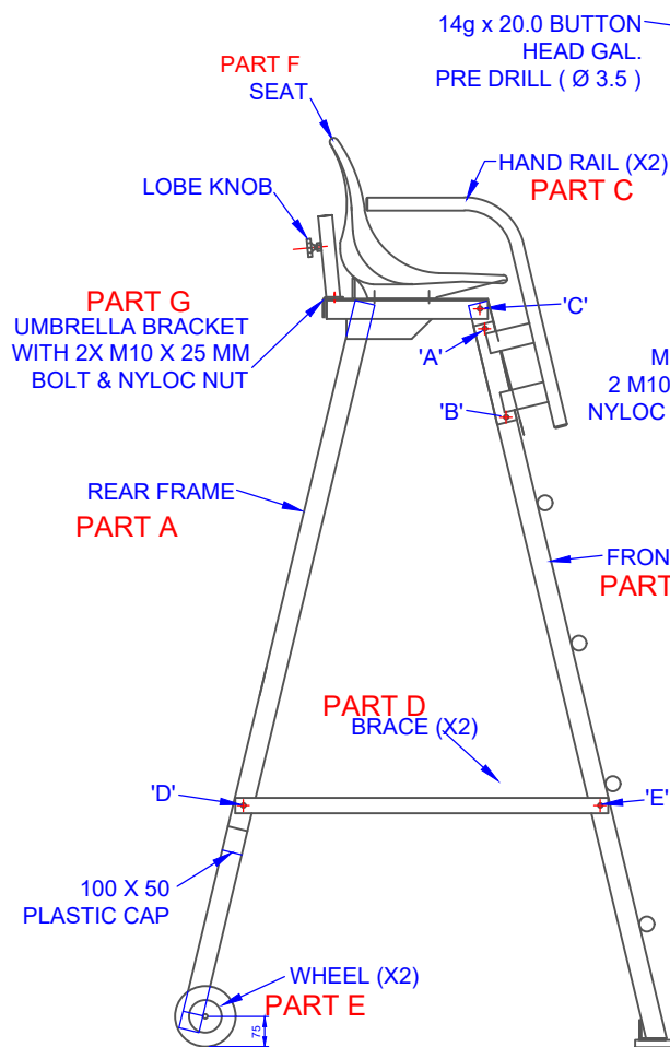
TC25 SEAT DETAIL
