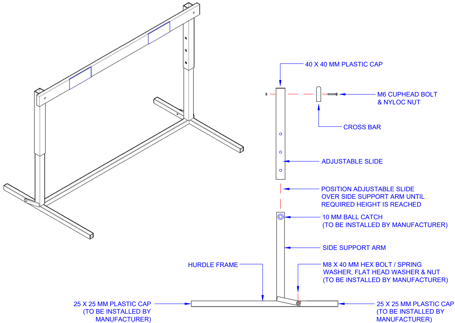
THD26 HURDLE SIDE VIEW SCALE 1:10
