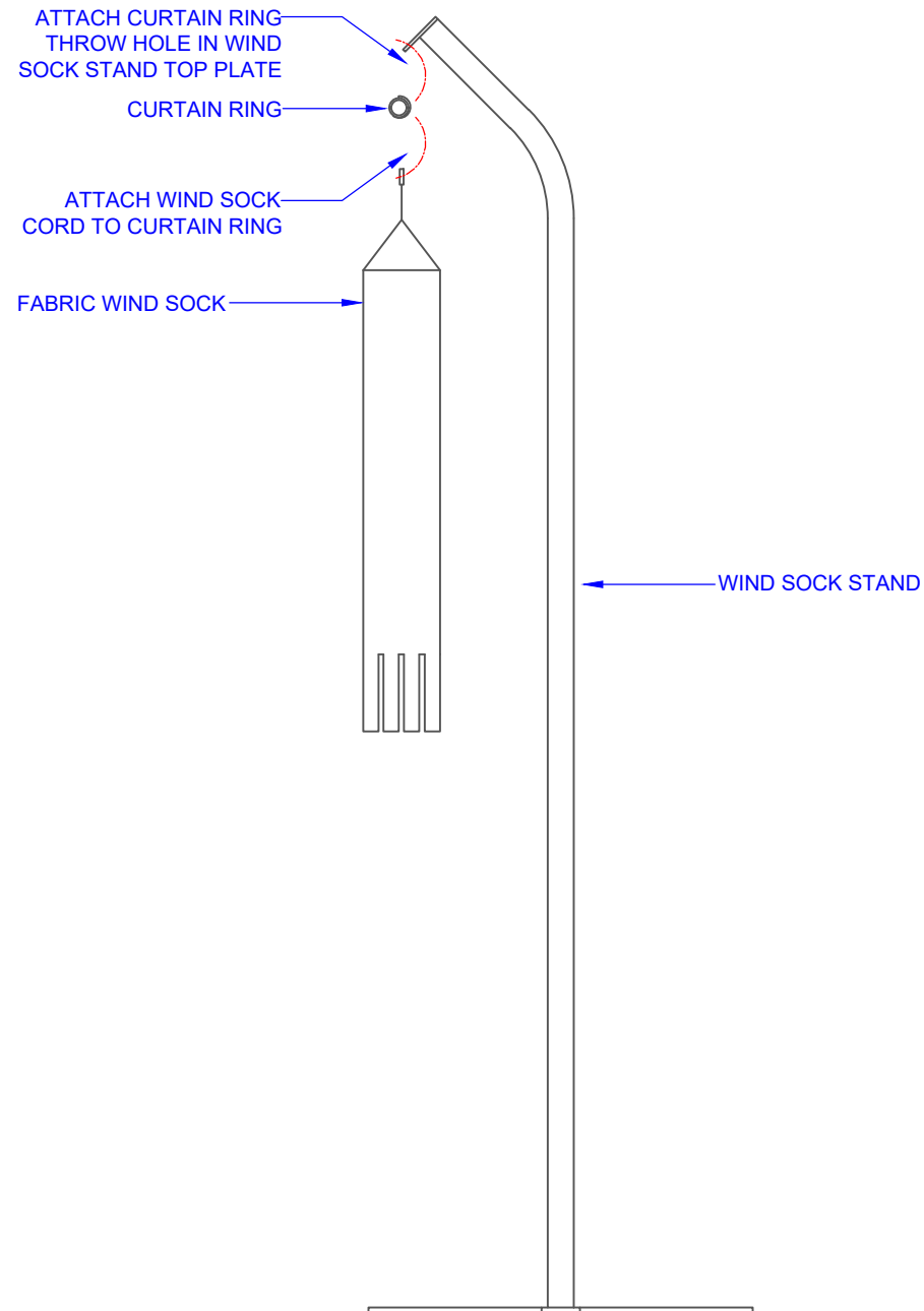
TMS55 WIND SOCK SCALE 1:10
