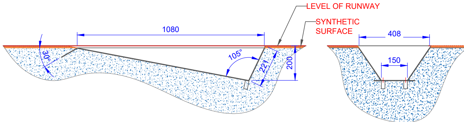
TPV15 POLE VAULT TROUGH
