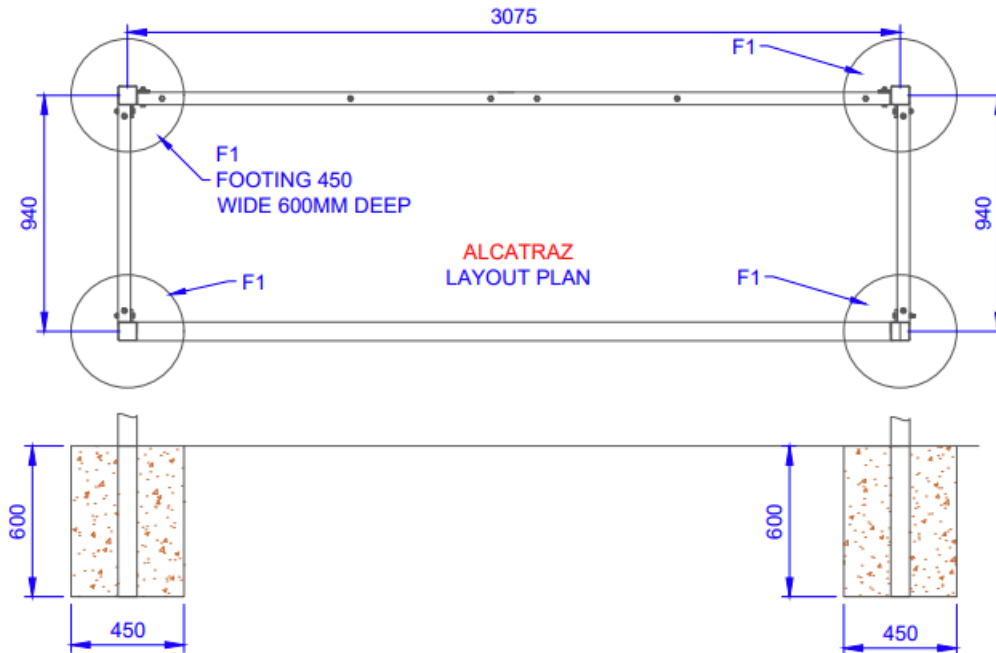
Fig: Alcatraz Footing Details
